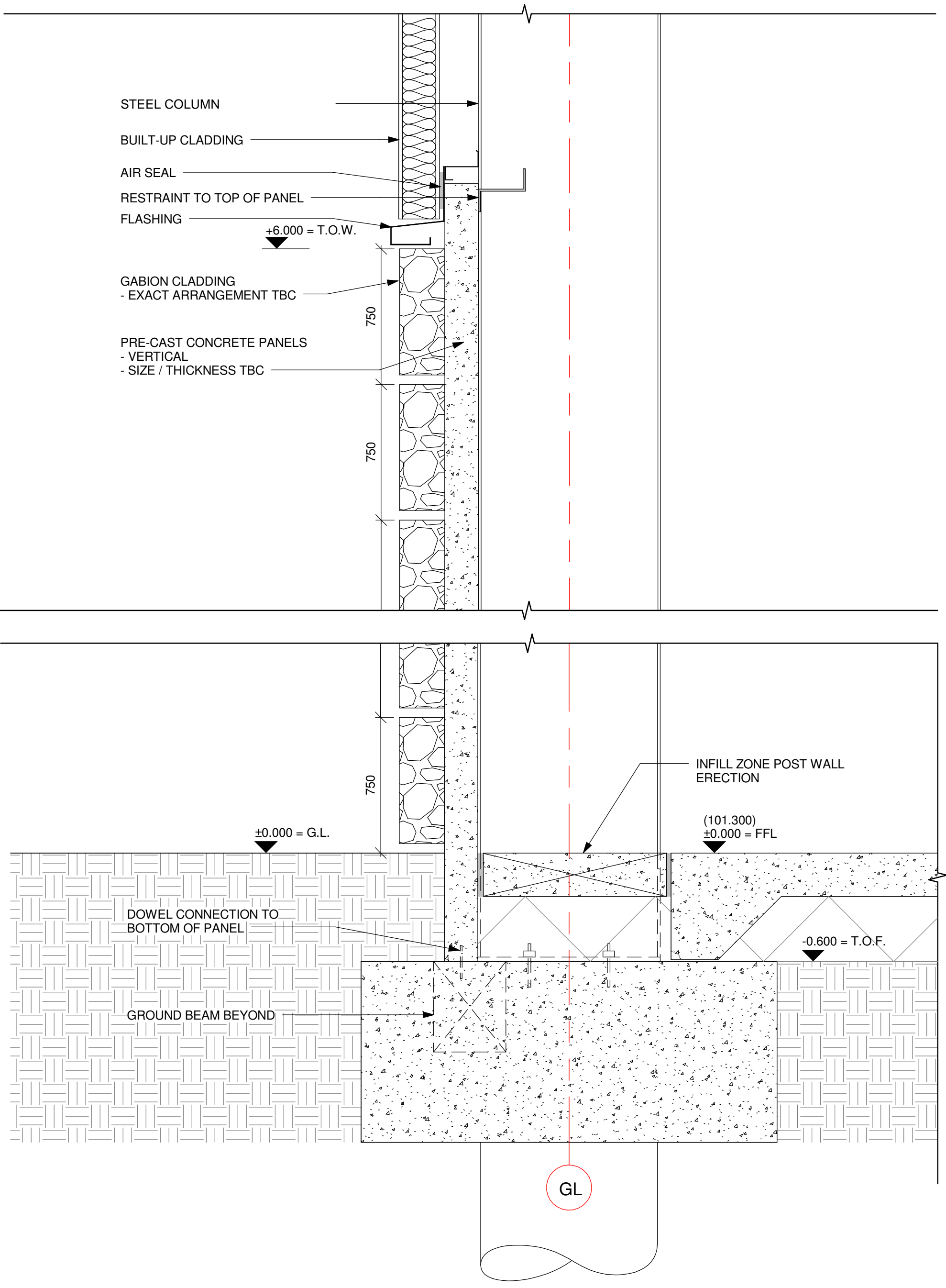
EXTERNAL WALL SECTION OF STEEL PROJECTS
